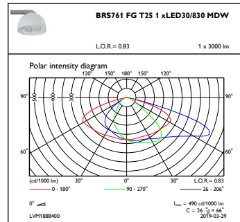
OFPC1_BRS761FGT251xLED30830MDW
