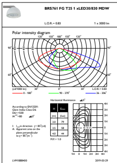
OFPL1_BRS761FGT251xLED30830MDW
